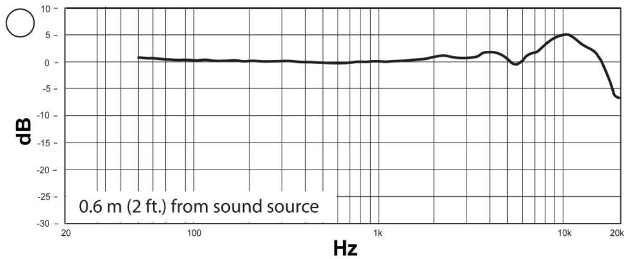
Omnidirectional
