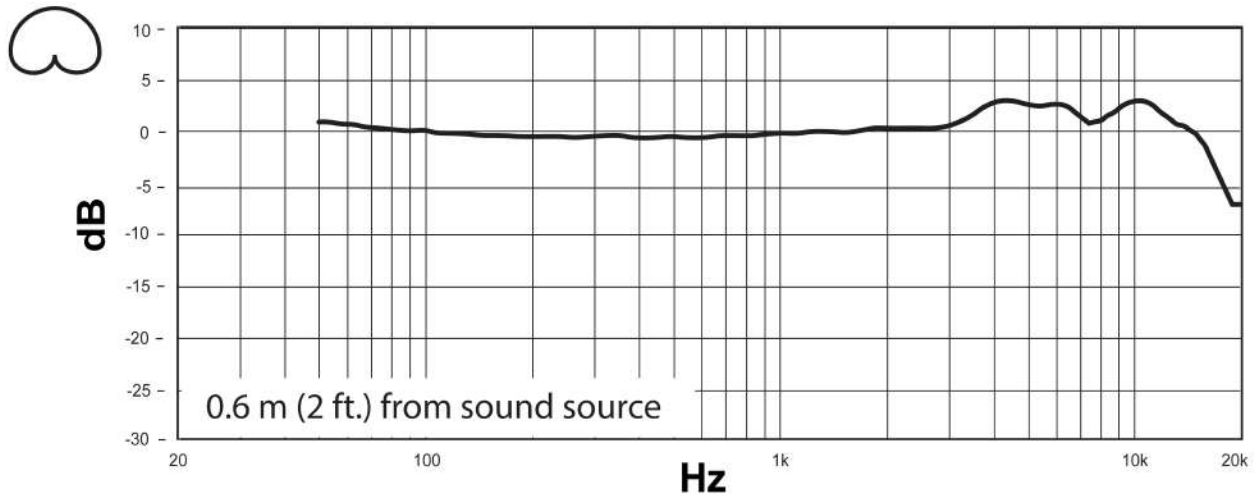
Cardioid
