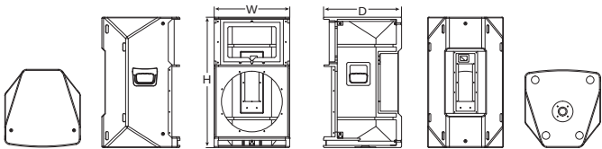
Dimension(W×H×D):439×760×454mm
