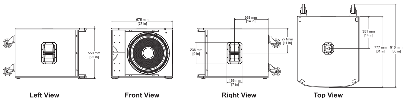
Figure 3.6: ETX-18SP dimension drawing
