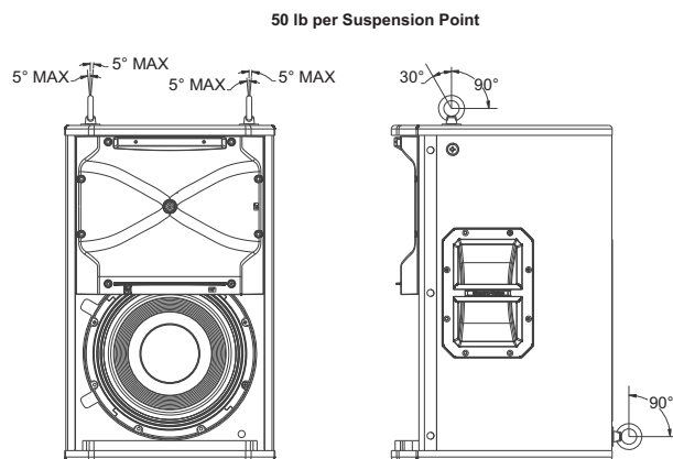
Figure 4.10: Maximum working load - vertical orientation
