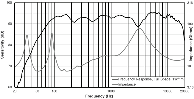
Frequency response and impedance:
