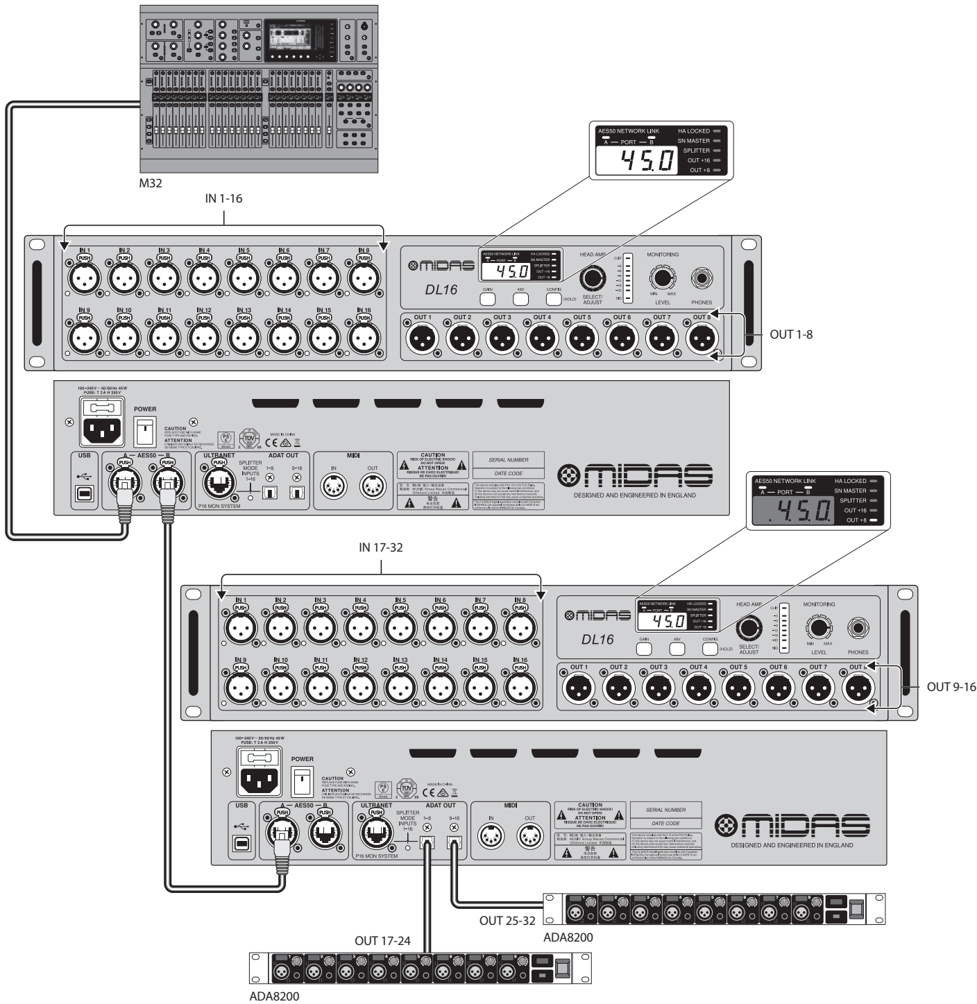
Linking two DL16 units
