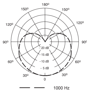
Polar Pattern
